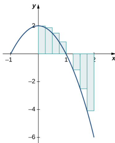
Figure 5.17 For a function that is partly negative, the Riemann sum is the area of the rectangles above the x -axis less the area of the rectangles below the x -axis.
