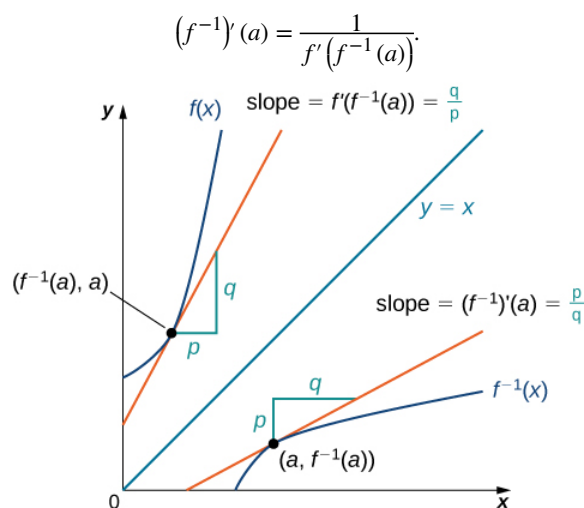
Figure 3.28 The tangent lines of a function and its inverse are related; so, too, are the derivatives of these functions.
