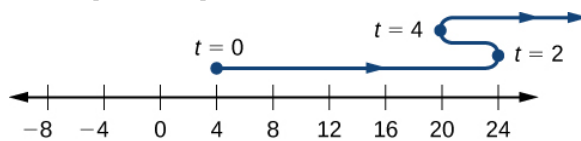
Figure 3.24 The path of the particle can be determined by analyzing v(t) .
