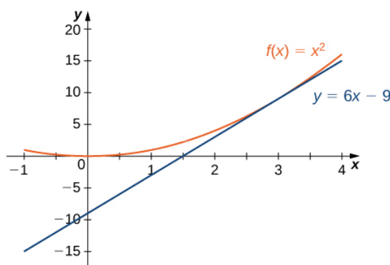
Figure 3.6 The tangent line to f(x) at x = 3 .
