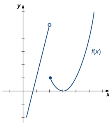
Figure 2.26 This graph shows a function f(x) .
