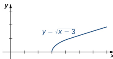
Figure 2.25 The graph shows the function f(x) = \sqrt{x-3} .
