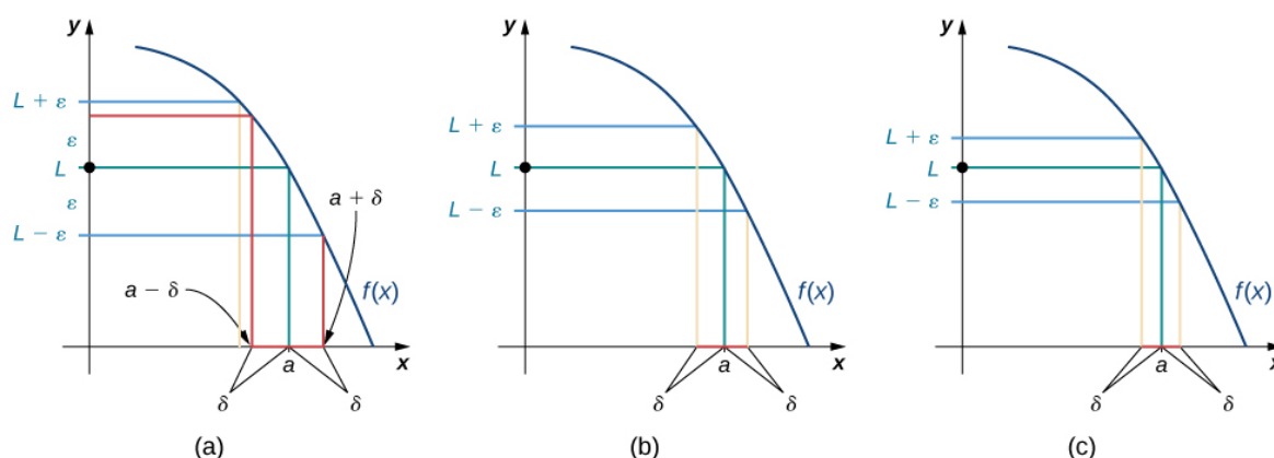
Figure 2.39 These graphs show possible values of \delta , given successively smaller choices of \varepsilon .
