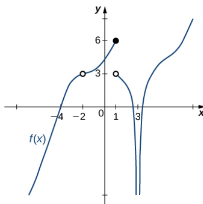
Figure 2.21 The graph shows f(x) .
