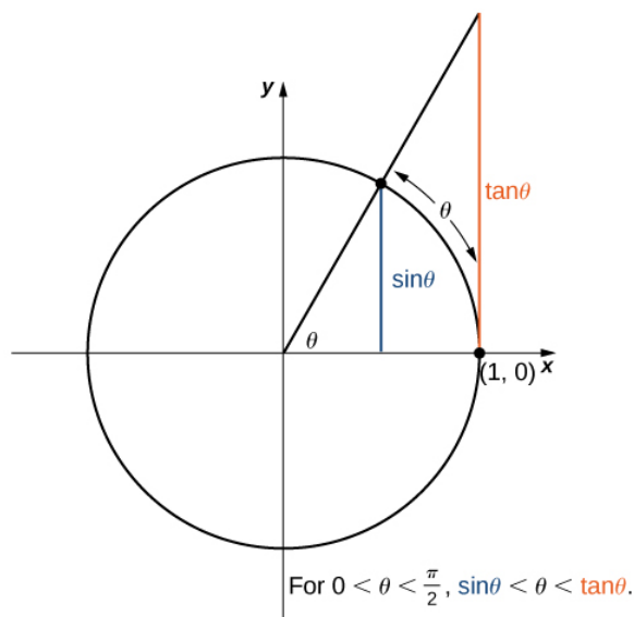
Figure 2.30 The sine and tangent functions are shown as lines on the unit circle.
