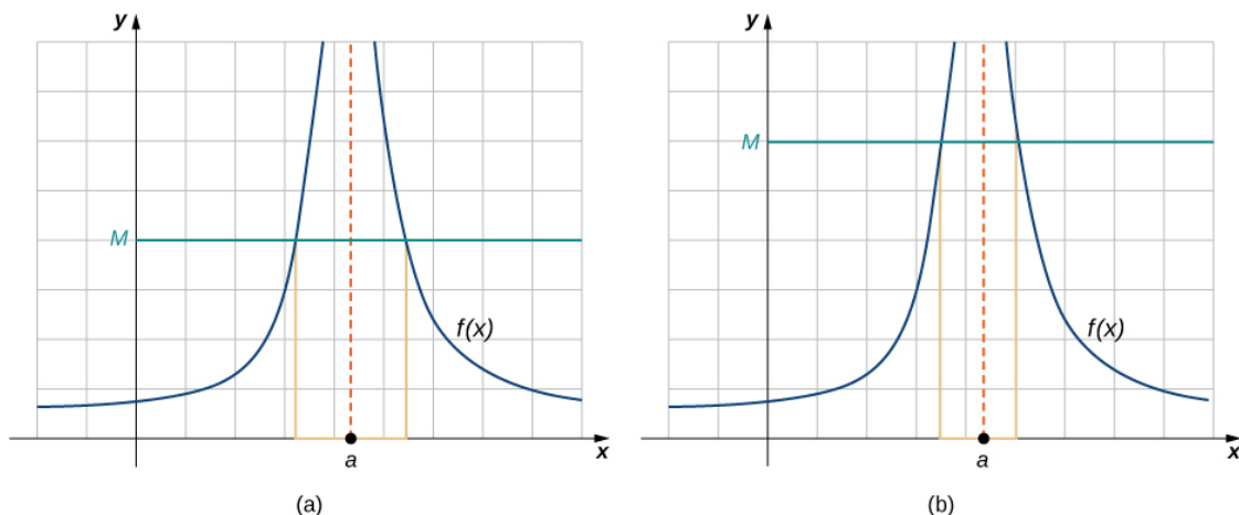
Figure 2.43 These graphs plot values of \delta for M to show that \lim_{x \rightarrow a} f(x) = +\infty .
